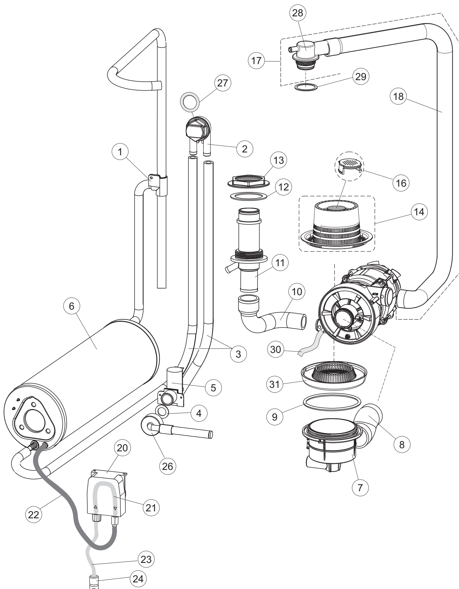
Drain Pump
